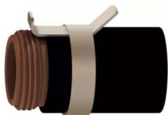
Hypertherm® Retaining Cap (Ohmic) 15 A - 105 A
